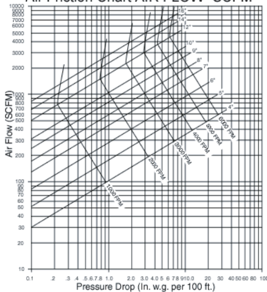
Air Friction Chart AIR FLOW "SCFM"*
